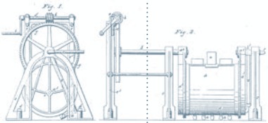
No. 16,082. H. BESSEMER. IMPROVEMENT IN THE MANUFACTURE OF STEEL. Patented Nov. 11, 1856.
